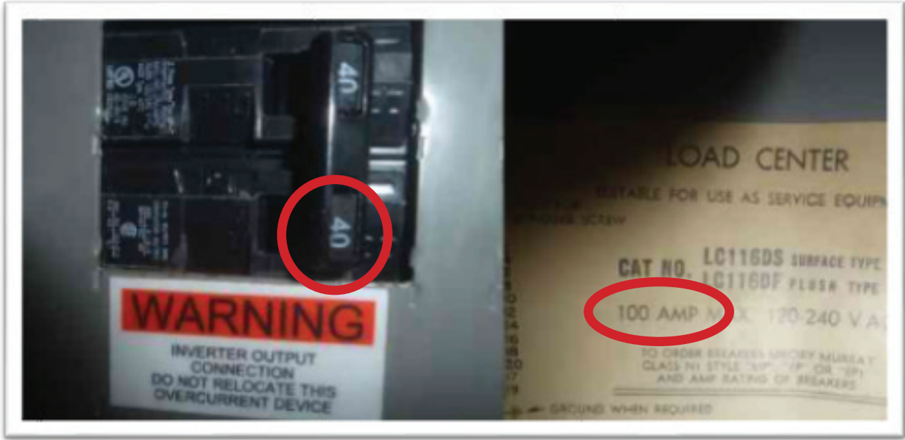
Photo D1: Main service panel overloaded per NEC 705(D)(2)(3)(b). (100 amp main circuit breaker + 40 amps of PV) ÷ 100 amp bus rating >120%.
