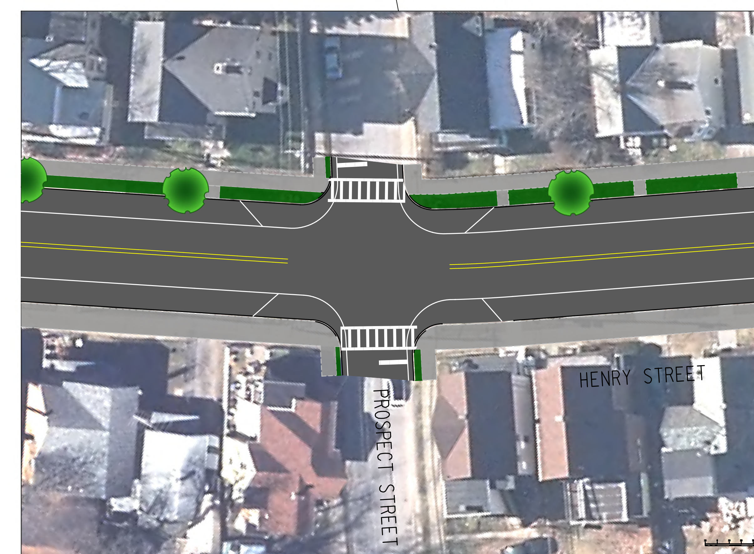
STRIPED CURB EXTENSION DETAIL PROSPECT STREET INTERSECTION
