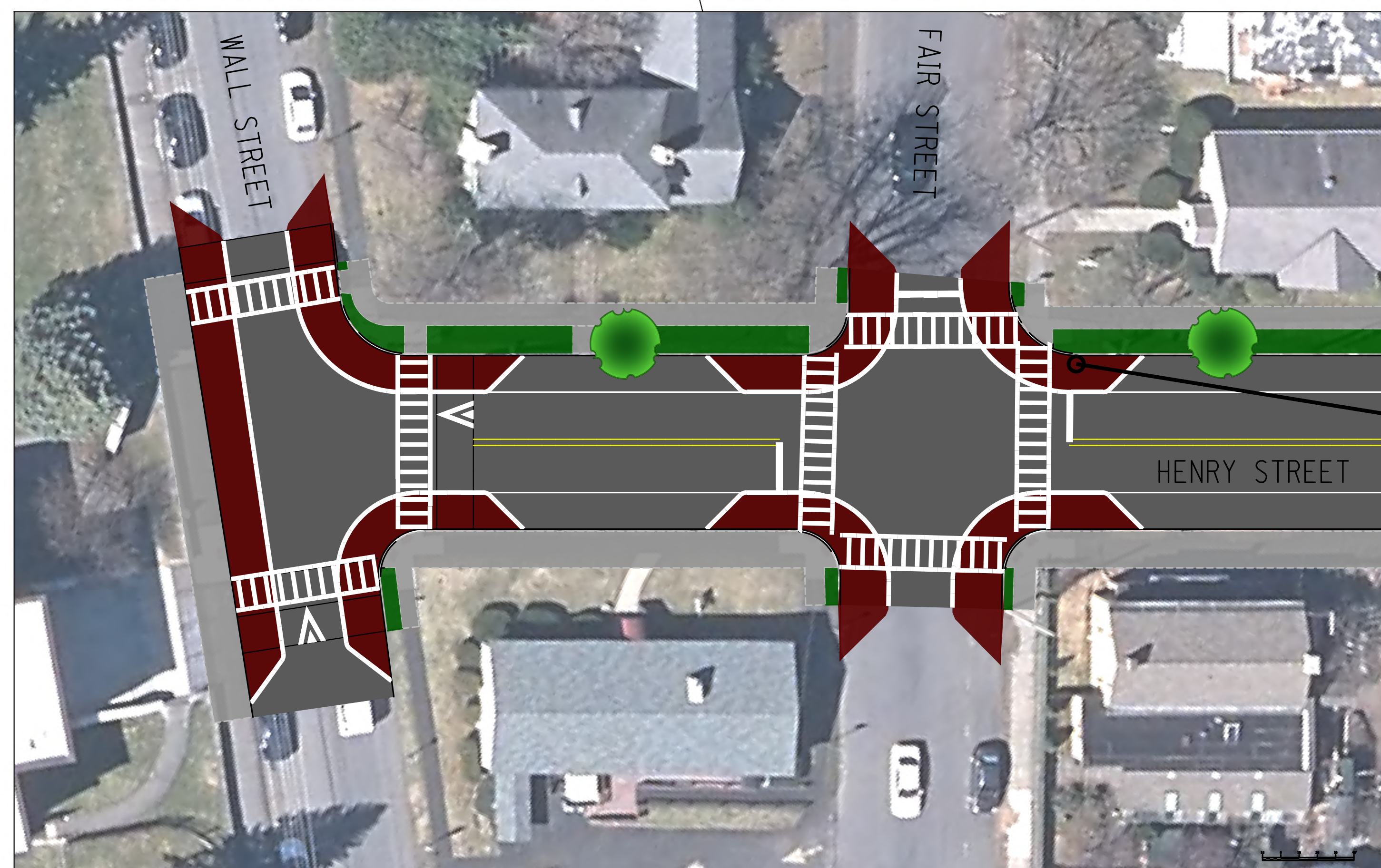
RED TEXTURED CURB EXTENSION DETAIL WALL STREET AND FAIR STREET INTERSECTIONS
